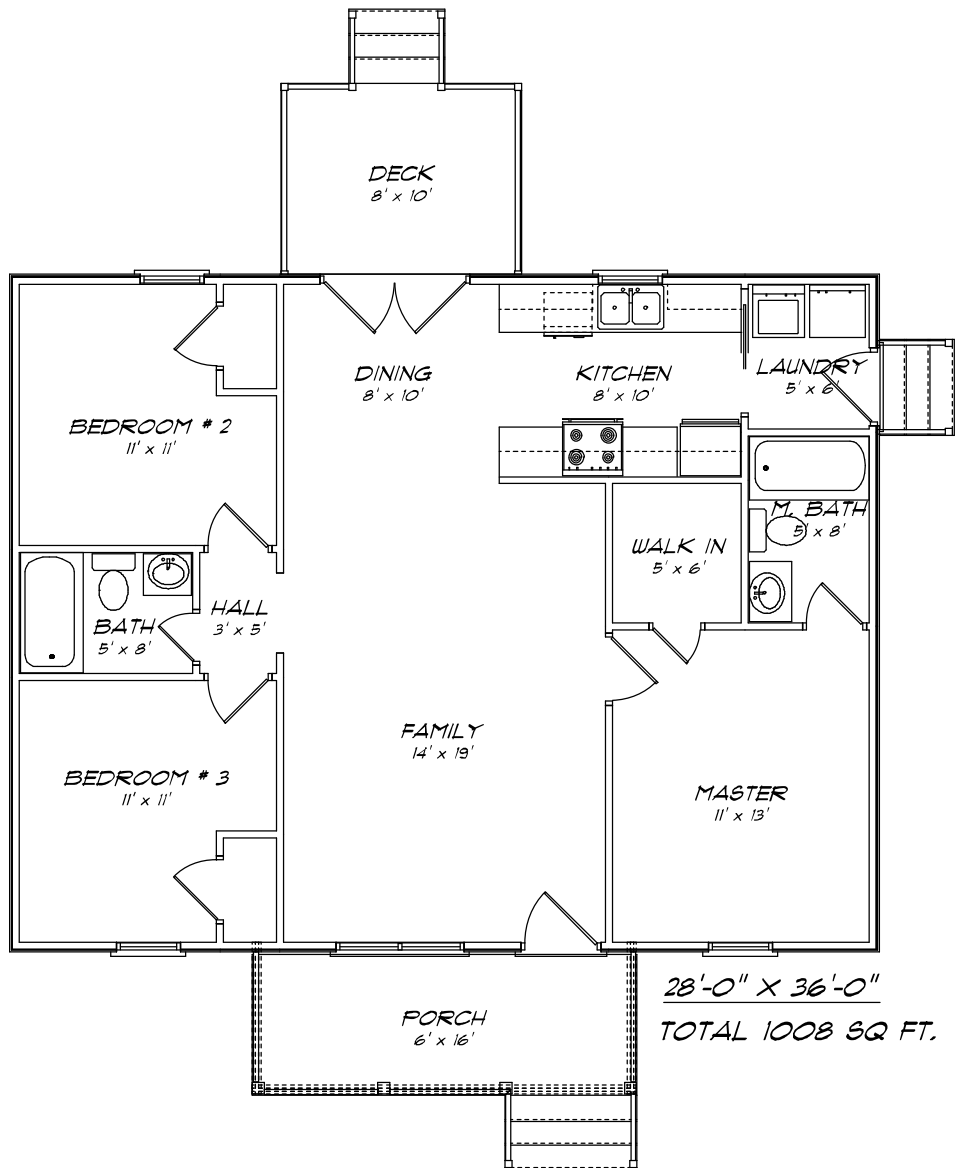
THE KEYSTONE I 1008 SQ. FT. 3 BED 2 BATH
