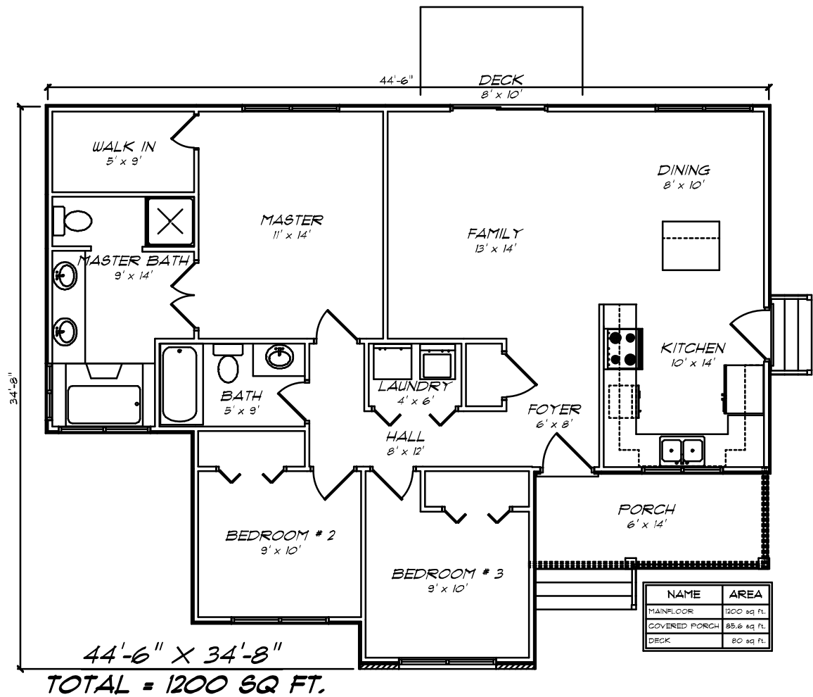
THE LAURA LYNN 1200 SQ FT 3 BED / 2 BATH
